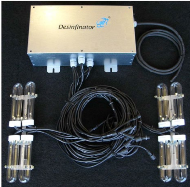
Externally mounted Control Module shown with 2 Slimline degreaser lamp modules
